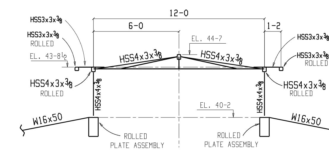
SECTION F
