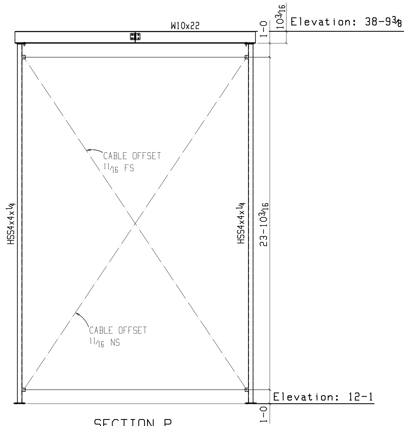
SECTION P
