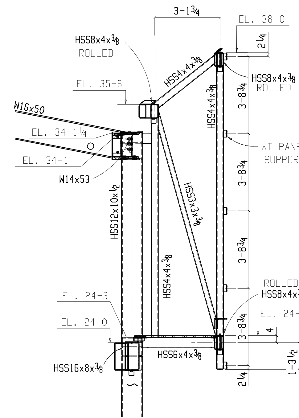
SECTION A
