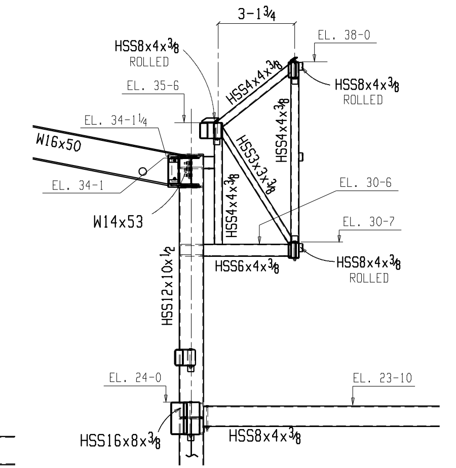
SECTION D
