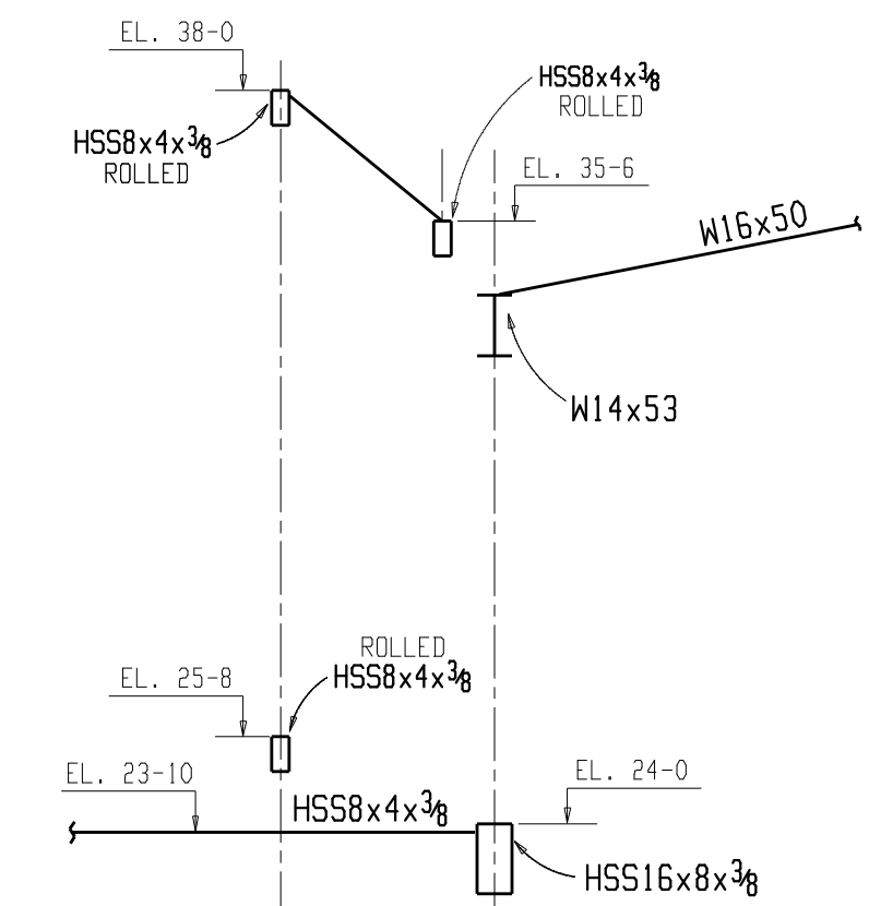
SECTION E
