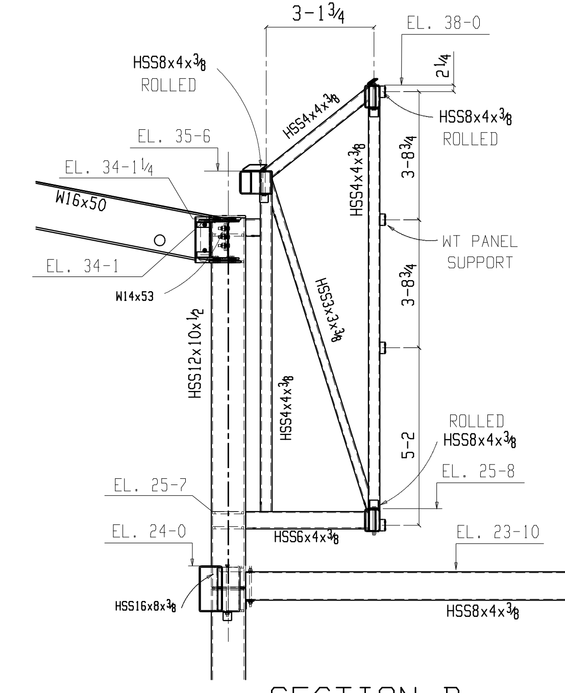
SECTION B
