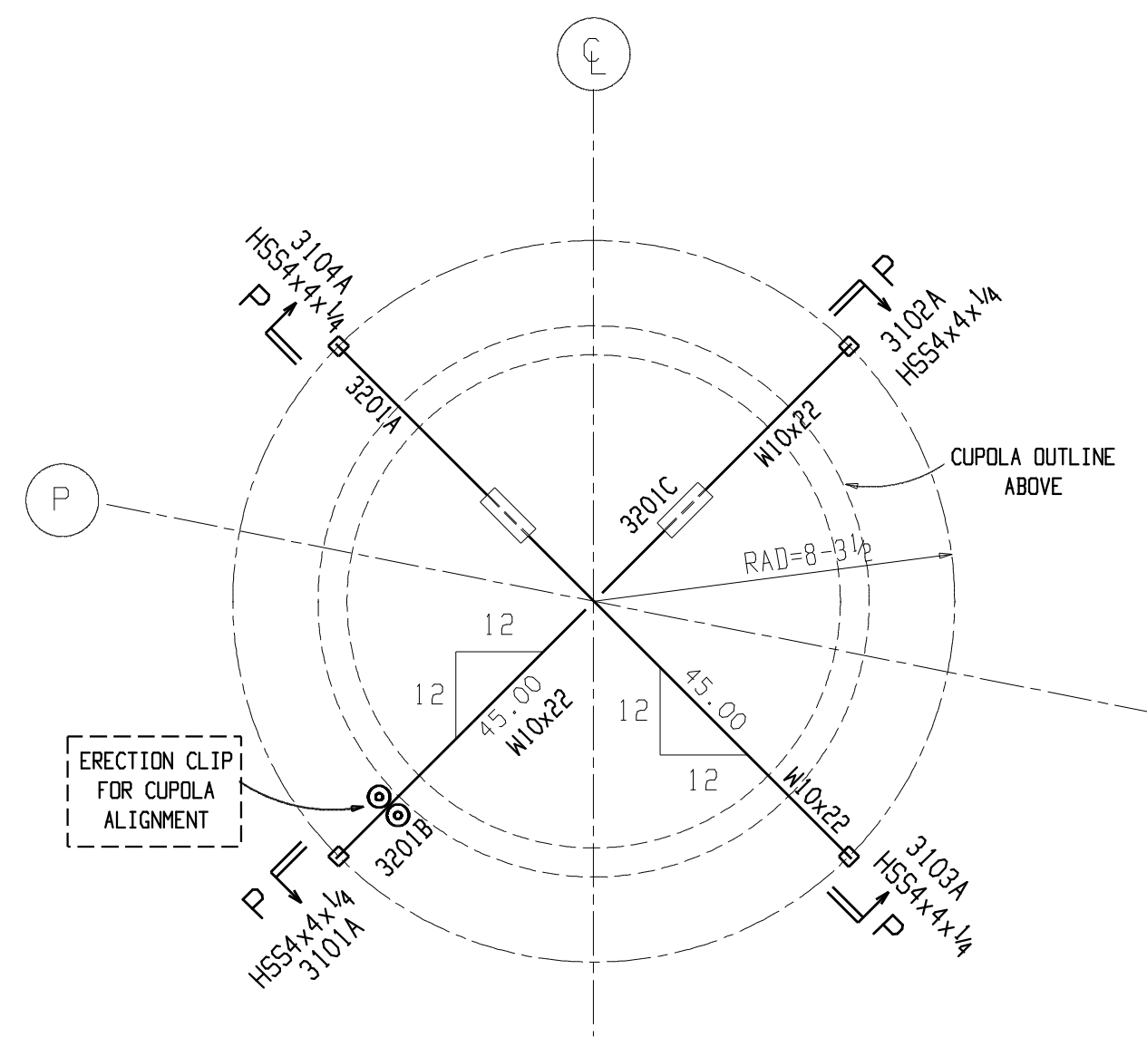
TEMPORARY CUPOLA ROOF SUPPORT PART PLAN
