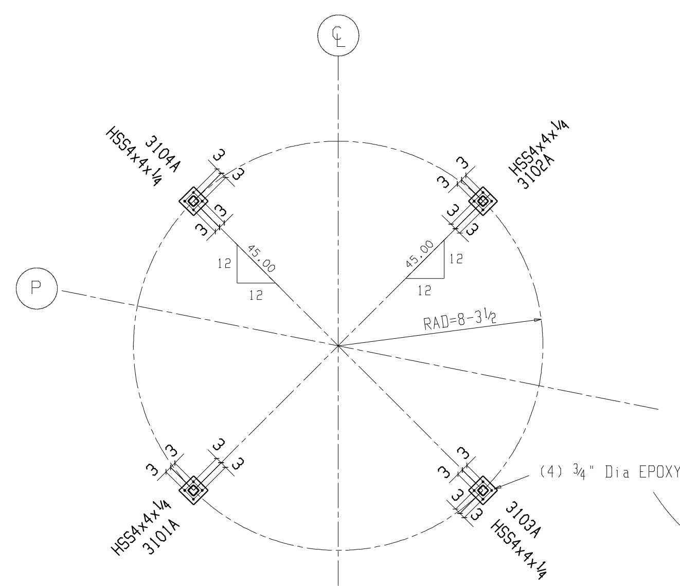
TEMPORARY CUPOLA ROOF SUPPORT AB PART PLAN
