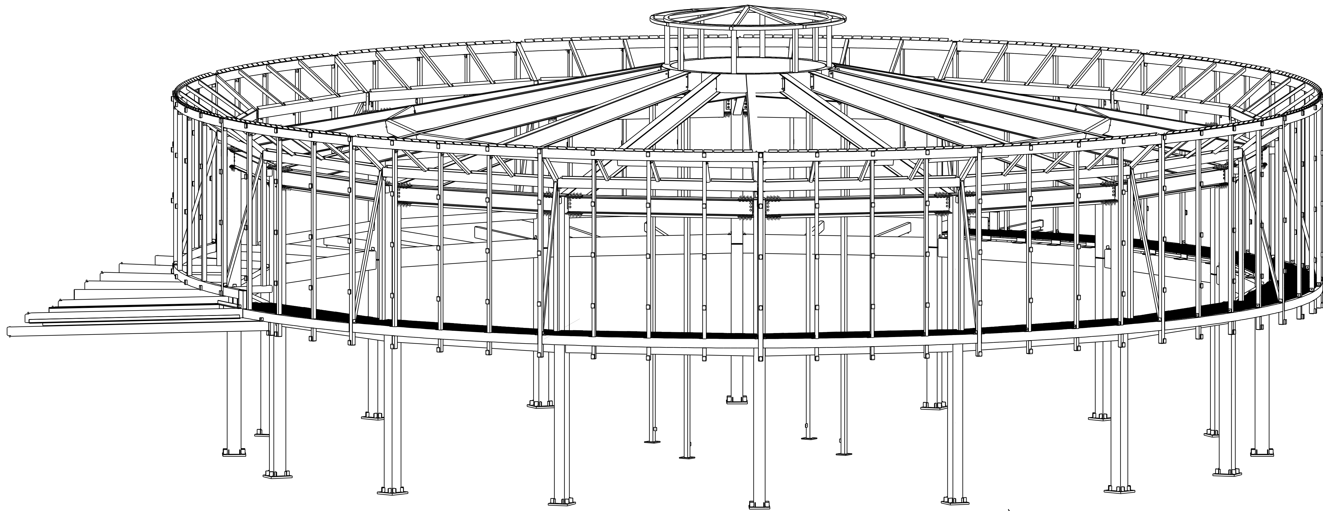
CAROUSEL ISO VIEW -SEQUENCE#3-
