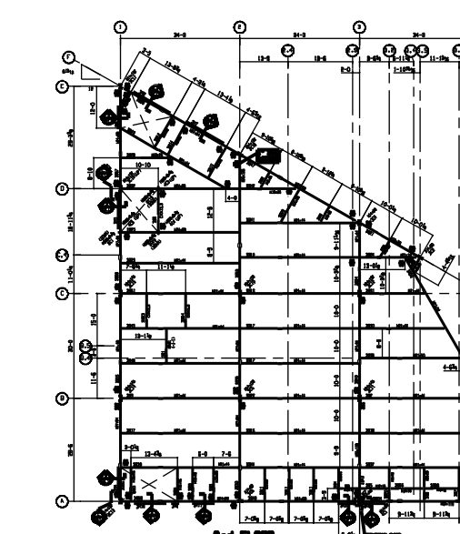
3rd Floor
