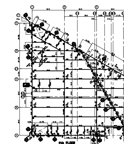
4th Floor
