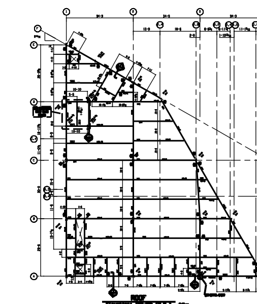
Roof
