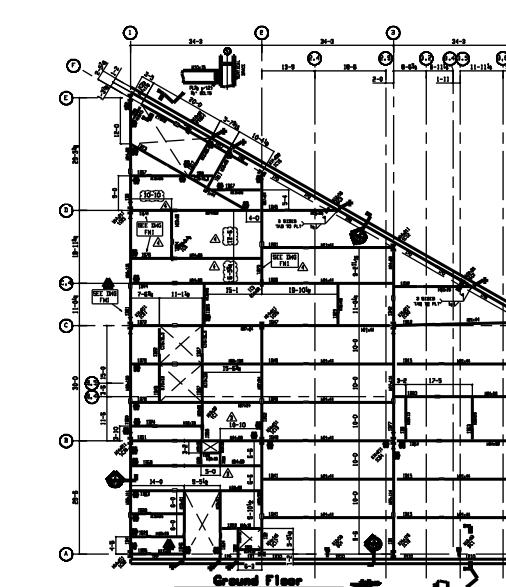
2nd Floor
